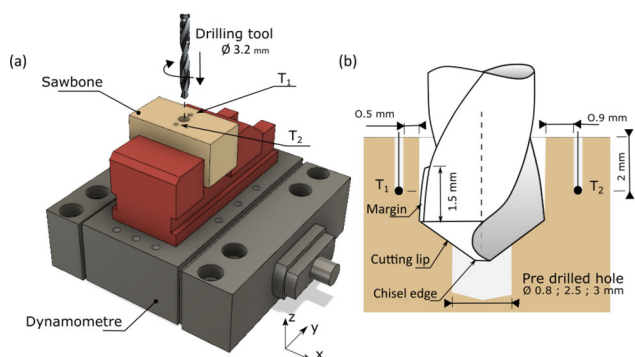
Figure 1. Experimental setup.
