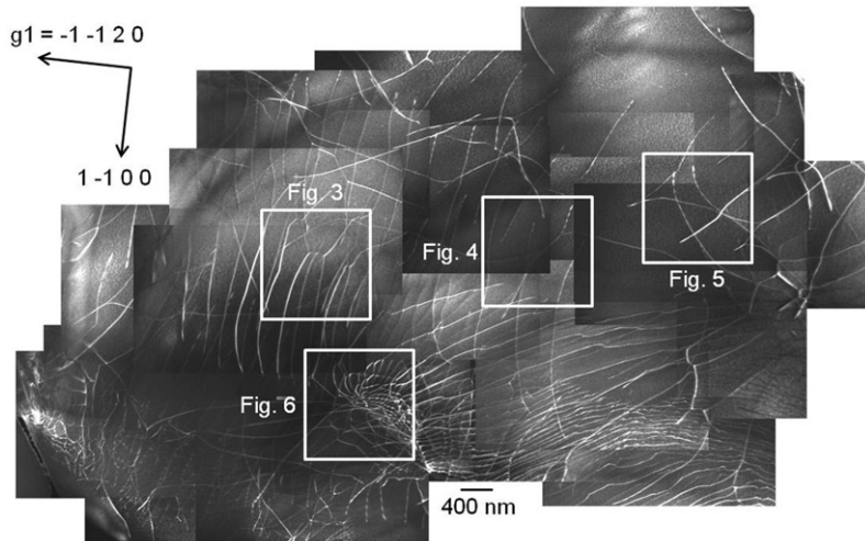
Figure 2. TEM micrograph showing a typical landscape observed in deformed \text{Ti}_2\text{AlN} , viewed using the diffracting vector g_1 = -1-120 in the (0001) zone axis. The white squares localise the studied areas presented in Figures 3, 4, 5 and 6.
