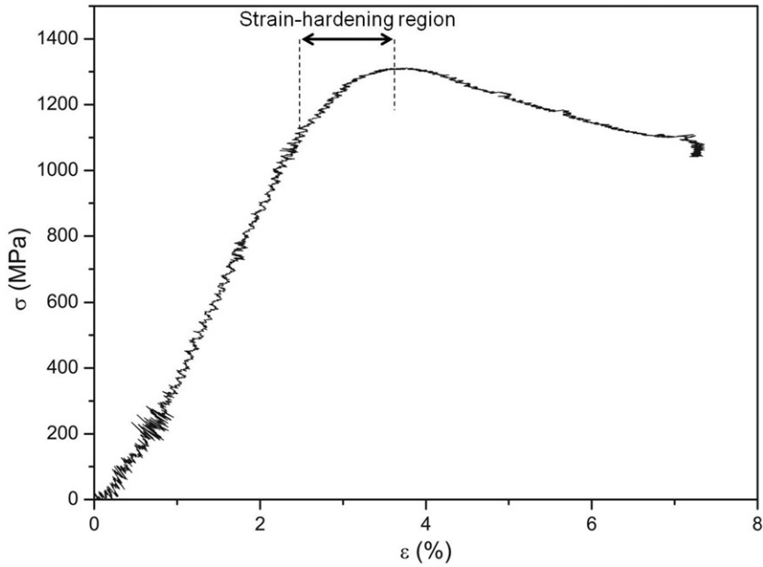
Figure 1. Stress–strain curve of \text{Ti}_2\text{AlN} deformed at room temperature under confining pressure (320 MPa).
