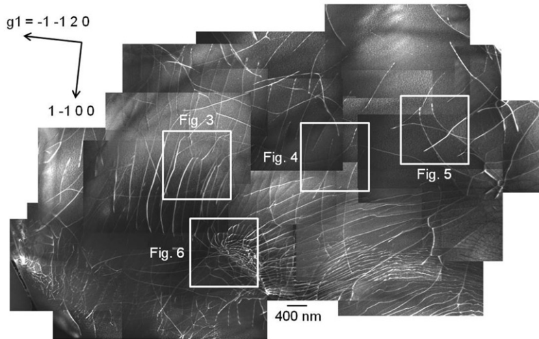
Figure 2. TEM micrograph showing a typical landscape observed in deformed \text{Ti}_2\text{AlN} , viewed using the diffracting vector \mathbf{g}_1 = -1-120 in the (0001) zone axis. The white squares localise the studied areas presented in Figures 3, 4, 5 and 6.
