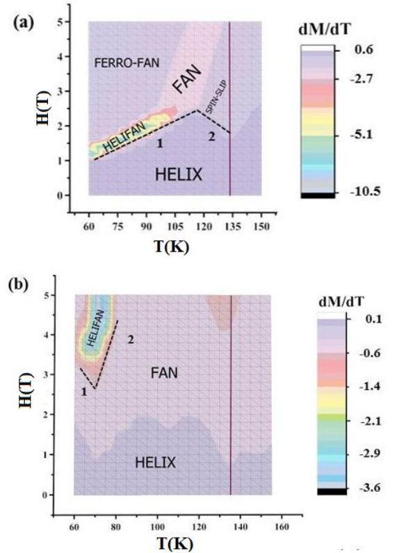
FIG.8. Magnetic phase diagram of W/Ho/W/MgO sample for in-plane (a), out-of-plane (b) field orientations. The lines 1 and 2 correspond to helifan-helix and spin-slip-helix transitions.
