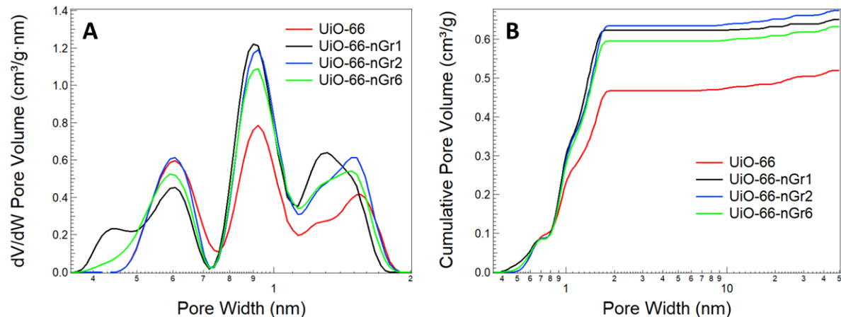
Figure 4. Differential pore size distributions calculated from N_2 isotherms using the 2D-NLDFT up to 2 nm (A) and cumulative pore volume (B).
