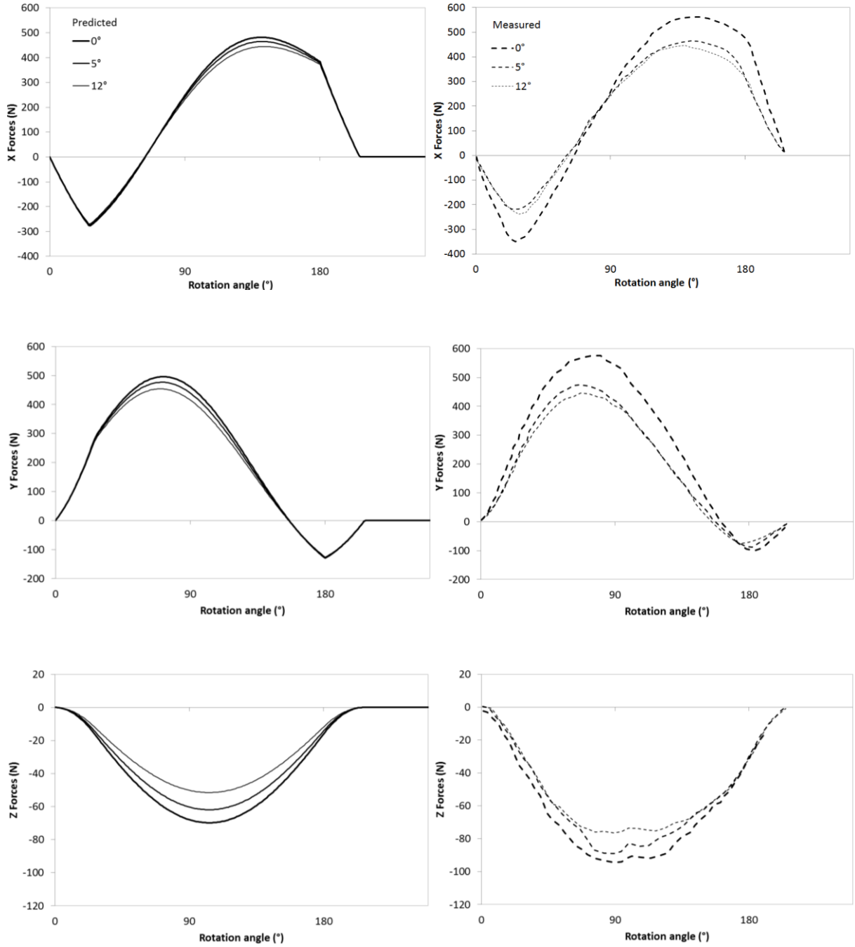
Fig. 6. Measured (from Yucesan and Altintas [9]) and predicted cutting forces for full immersion tests and for various rake angle values \alpha_r = 0^\circ, 5^\circ and 12^\circ . Single-fluted end mill, feed rate f_t = 0.0127 \text{ mm/tooth} , axial depth of cut d_a = 7.5 \text{ mm} , cutting speed V = 30 \text{ m/min} .
