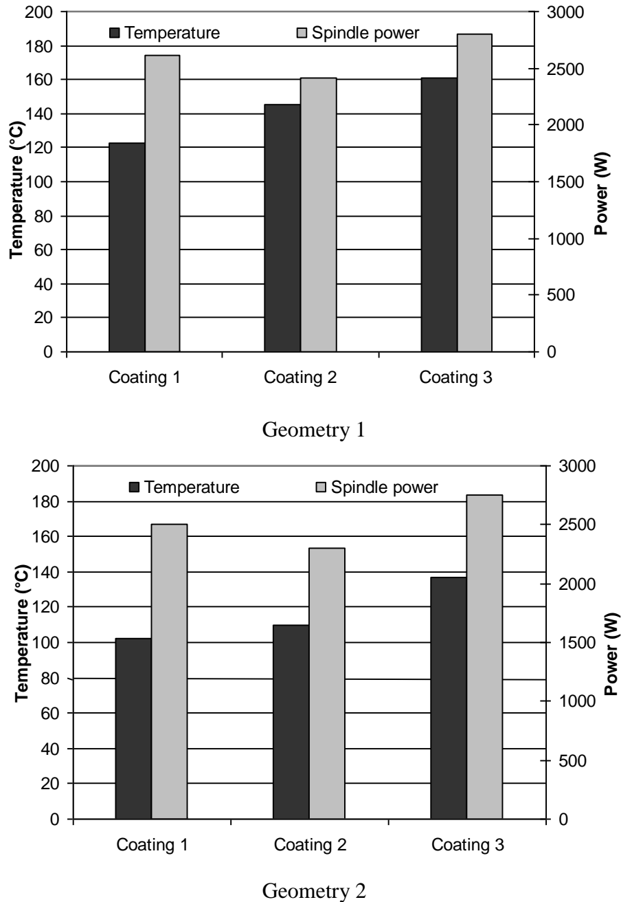
Figure 6. Maximum temperature and spindle power for tool geometries 1 and 2.
