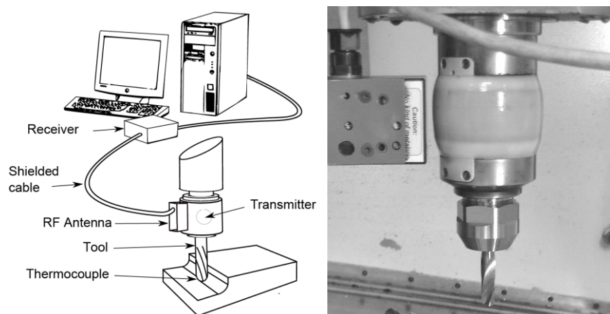
Figure 1. Tool holder, RF Antenna and data acquisition diagram.
