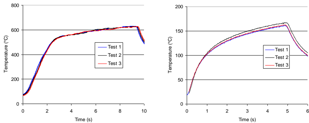
(a) drilling Ti6Al4V
