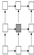
Fig. 9. Local network for the protocol \mathcal{P}_{3,n}^{ij}
