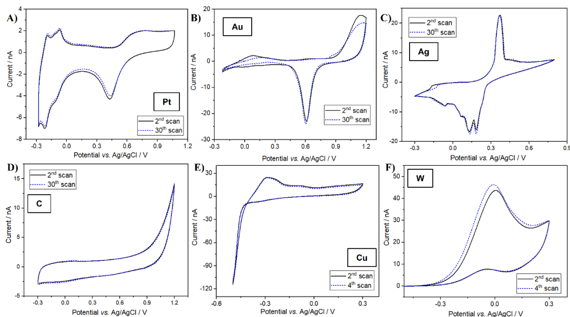
Figure 4. CVs of 3D printed microelectrodes in 0.1 mol/L \text{H}_2\text{SO}_4 (for Pt, Au, Ag and C) or PBS ( \text{pH} = 7.4 , for Cu and W).
