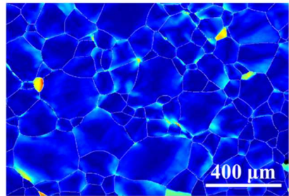
Deformation of \beta grains
