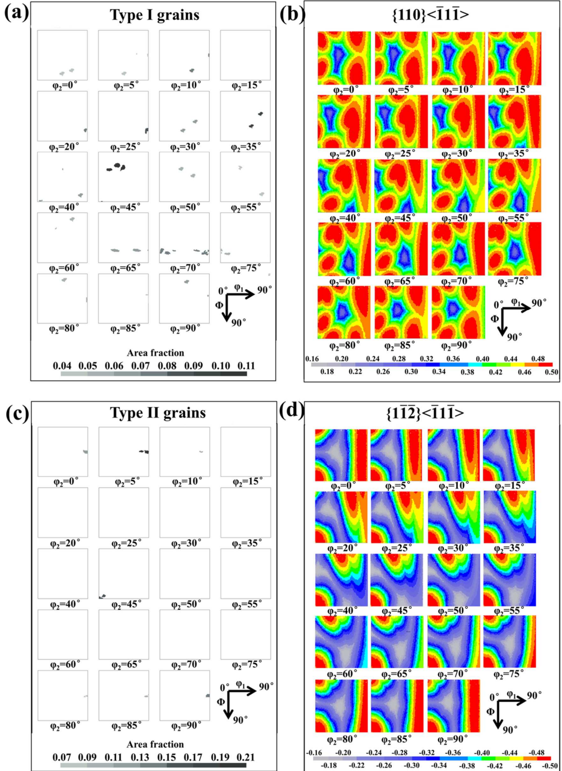
Fig. 10 (a) and (c) \phi_2 sections of the measured orientations of the respective type I and type II \beta grains normalized with the total areas of the respective type of \beta grains and (b) and (d) calculated resolved shear stress of the unitary external compressive
