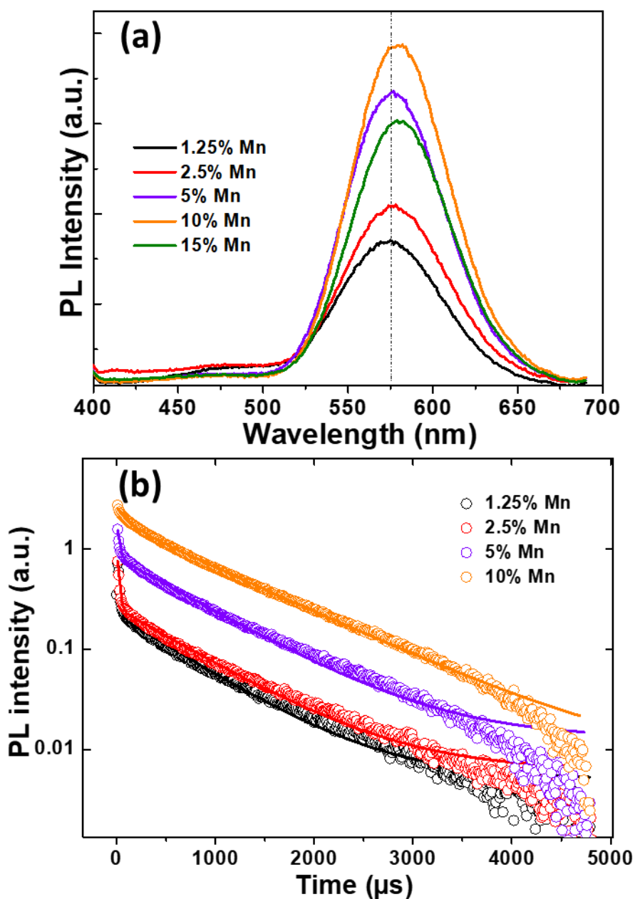
Fig. 3. (a) PL emission spectra of Mn:ZnSeS QDs when varying the \text{Mn}^{2+} dopant percentage (reactions were conducted at pH 7 and the heating time was fixed at 7 h), (b) PL decay curves of Mn:ZnSeS QDs when varying the \text{Mn}^{2+} loading. Spectra were recorded at the maximum emission wavelength and an excitation of 355 nm was used.
