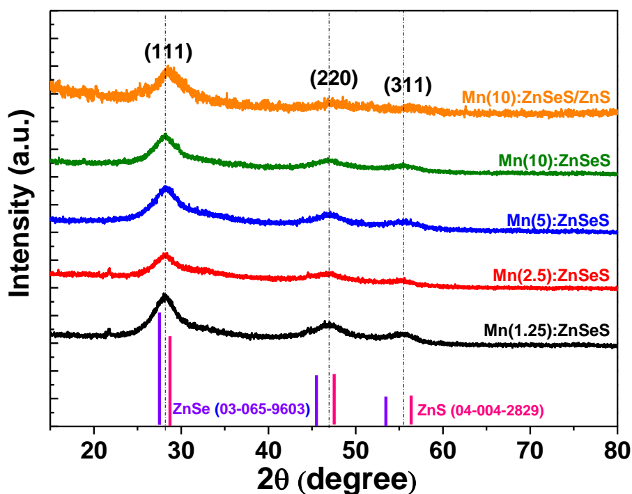
Fig. 6. XRD patterns of Mn:ZnSeS QDs when varying the Mn 2+ dopant percentage and of core/shell Mn(10):ZnSeS/ZnS QDs.
