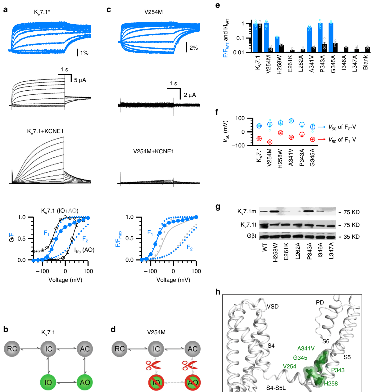
Fig. 1 Classic interactions are necessary for E-M coupling when the VSD transitions into the intermediate state. a VCF recordings of pseudo-WT K_{v}7.1^* ( K_{v}7.1 -C214A/G219C/C331A). K_{v}7.1 +KCNE1 currents are shown at the same scale. The F-V relationships (blue circles) are fitted with a double Boltzmann function. F_1 -V represents the VSD transition from resting to intermediate state; F_2 -V represents the VSD transition from the intermediate to activated state. G-V represents channel opening with VSD transition at both the intermediate (IO) and the activated (AO) states. b Cartoon scheme illustrating the gating mechanism of two-step VSD movements and distinct two open states. c VCF recordings of V254M in K_{v}7.1^* . V254M+KCNE1 currents are shown at the same scales. The F-V relationships of K_{v}7.1^* and V254M are shown in gray and blue, respectively. d Cartoon scheme illustrating that V254M disrupts E-M couplings for both IO and AO. e Summary of data for WT and mutant K_{v}7.1 . VSD activation (blue, percentage change in fluorescence) and pore opening (black, current amplitude) are normalized to the WT. n \geq 3 . Blank: cells not injected with channel mRNA. Data points are shown in small open circles. f V_{50} values for the F_1 -V and F_2 -V. n \geq 3 . Data points are shown in small open circles. g Western blot results showing the membrane (top) and total (middle) expression of some mutants that eliminated both fluorescence and ionic currents. G \beta (bottom) from total protein is shown as negative control. WT K_{v}7.1 , H258W, and P343A are shown as positive controls. h Mapping the key residues V254, H258, A341, P343, and G345 (green) onto the S4-S5L/S6c interface in the K_{v}7.1 cryoEM structure (PDB: 5VMS) 2 . All averaged data are shown in mean \pm SEM. Source data are provided as a Source Data file.
