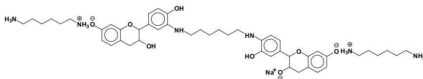
Figure 11. Example of covalent bonds dimer mixed with ionic salt bonds at 880 Da.
