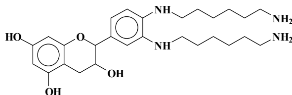
Figure 4. Example of covalent bonds structure at 509–512 Da.
