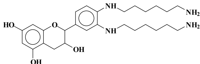
Figure 19. Covalently linked diamine onto catechin B-ring sites.
