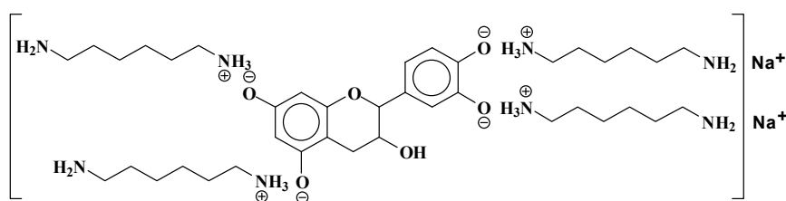
Figure 10. Example of ionic bonds salt structure at 798 Da.
