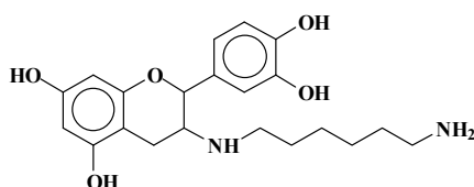
Figure 18. Covalently linked diamine onto \text{C}3 site of catechin.
