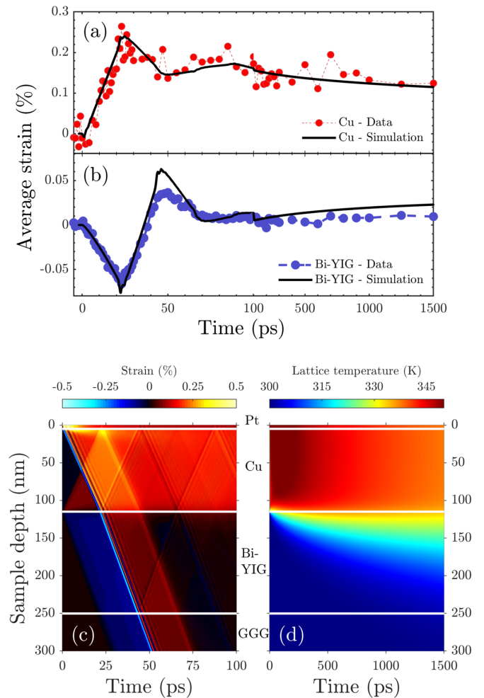
FIG. 1. Laser-induced lattice dynamics in the Pt/Cu/ \text{Bi}_1\text{Y}_2\text{Fe}_5\text{O}_{12} / \text{Gd}_3\text{Ga}_5\text{O}_{12} heterostructure. Average strain in (a) the Cu layer and (b) Bi-YIG layer as measured by ultrafast x-ray diffraction (UXRD). Calculated spatiotemporal maps of (c) the strain and (d) temperature in the heterostructure. The solid lines in (a) and (b) are results of our modeling. The UXRD measurements were performed at room temperature with a pump wavelength of 800 nm, a pulse duration of 50 fs, and an incident pump energy density of 5 \text{ mJ/cm}^2 .
