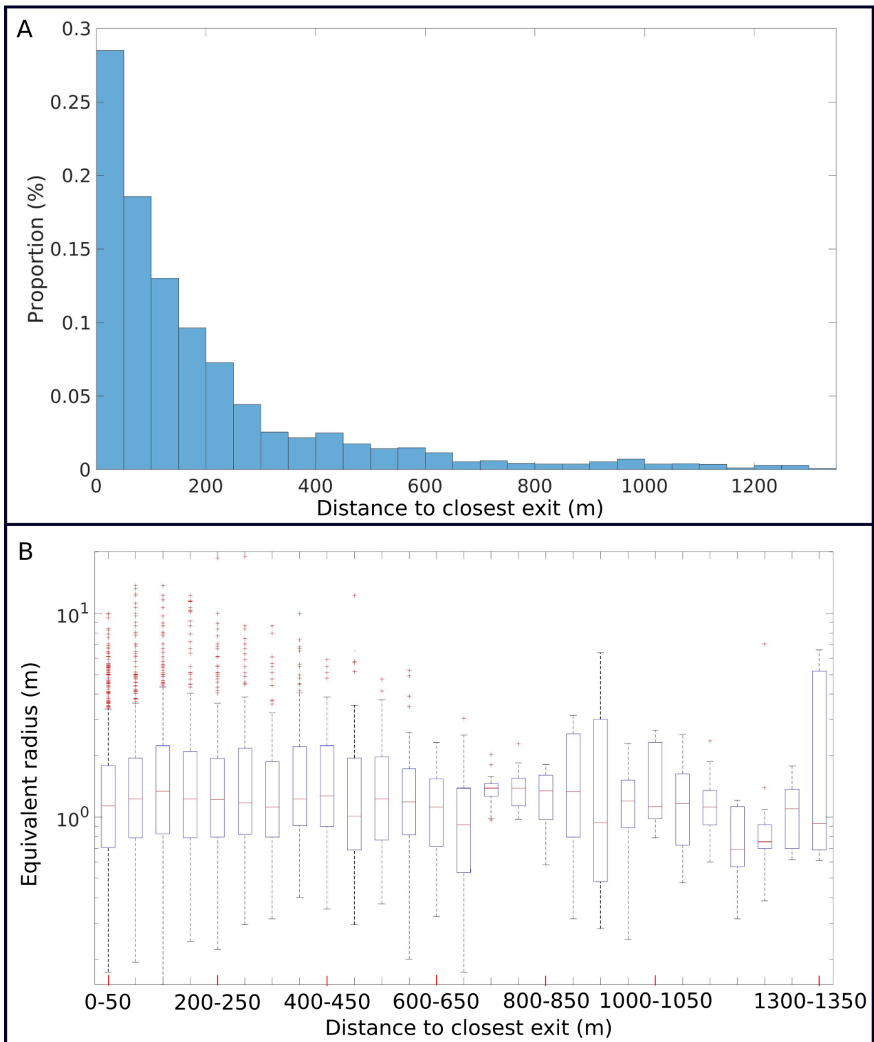
Figure 20 A: Histogram of the distance to the closest exit within the Arrestelia network (4283 nodes). B: Boxplot of the equivalent radius depending on the distance to the closest exit within the Arrestelia network.
