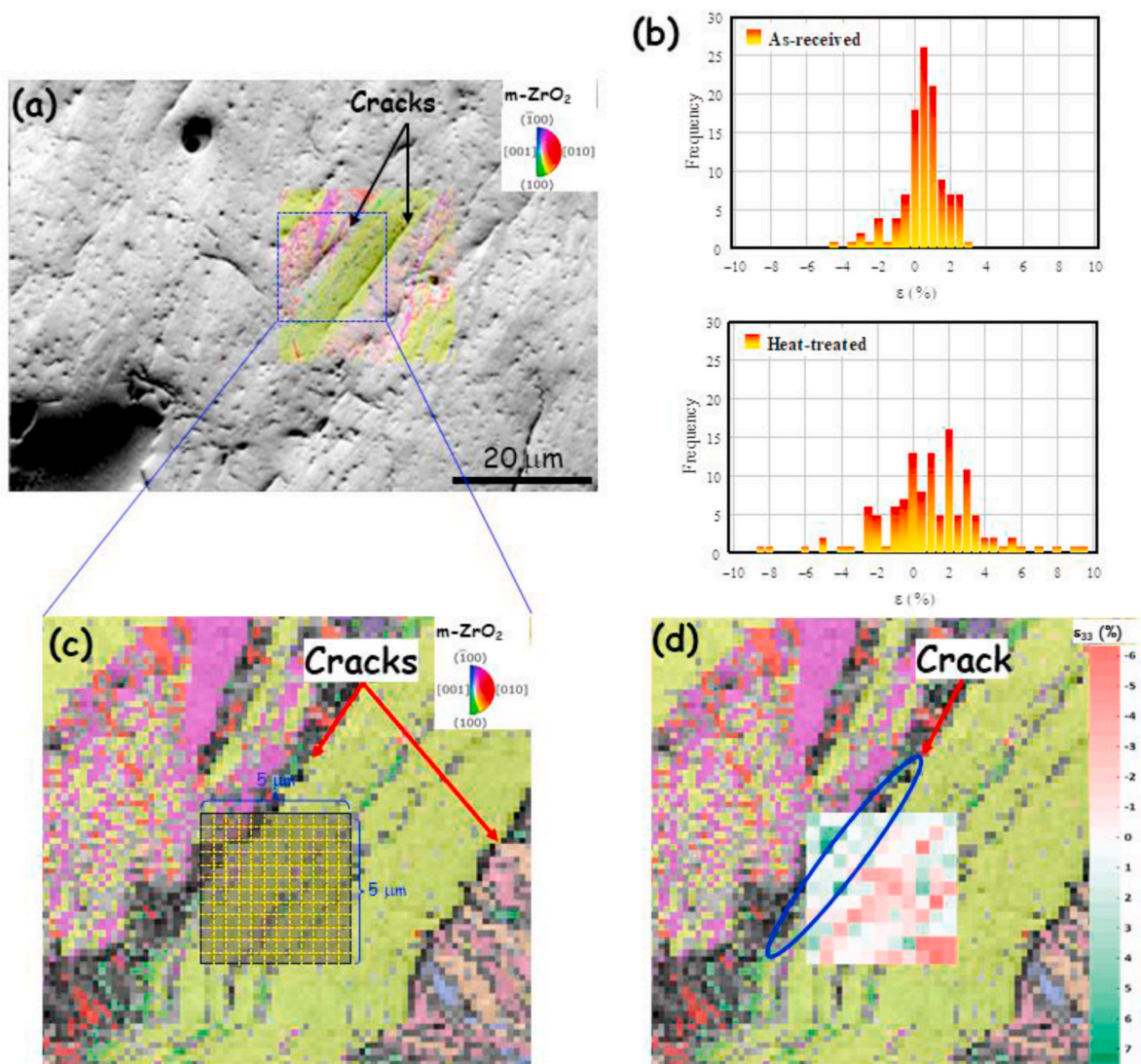
Fig. 5. Influence of a post-elaboration heat treatment at 1500 °C (Sample 2b). (a) SEM microstructure and Inverse Pole figure map obtained by EBSD. (b) Distribution of \varepsilon_{33} obtained by Laue microdiffraction, compared to sample 2a. (c) Mesh showing the area scanned by Laue microdiffraction. (d) Map of \varepsilon_{33} superimposed upon the EBSD map.
