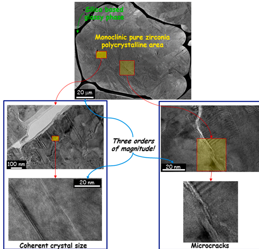
(a) Microstructure probed by electronic microscopy. The main picture was obtained by scanning electronic microscopy while the four smaller ones are transmission electron microscopy images evidencing both coherent domains and microcracks through high resolution observations.
