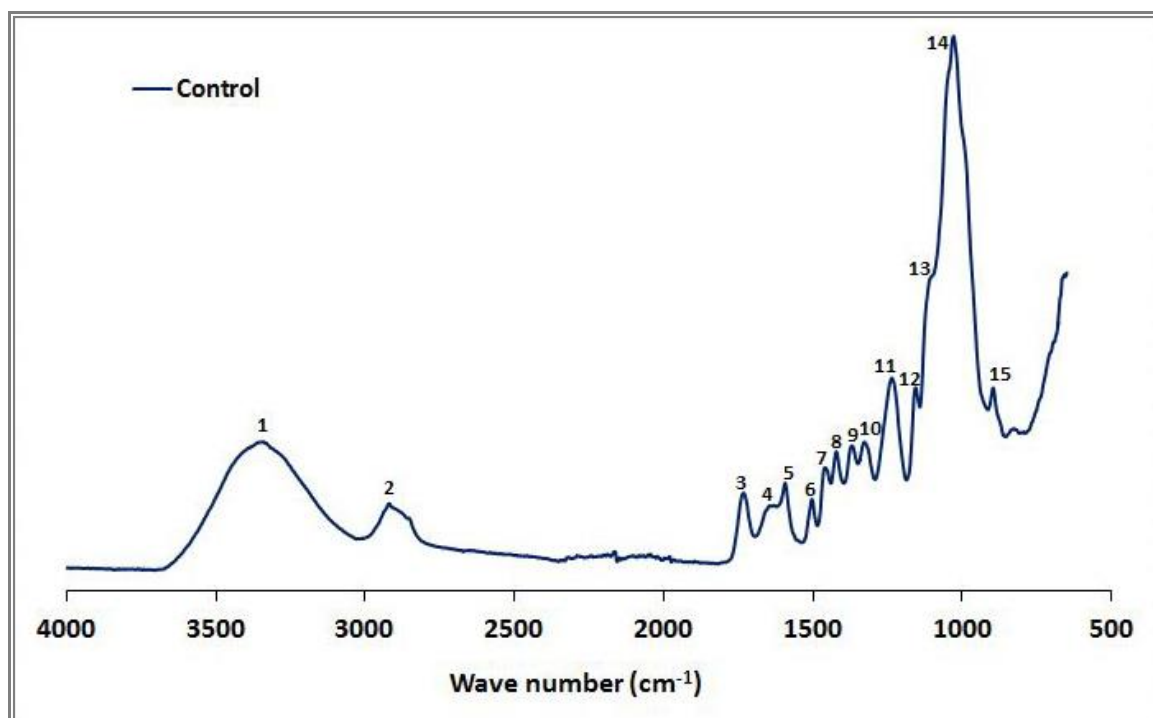
Figure 1. The IR spectra of the control beech wood.
