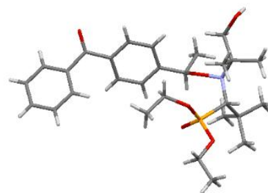
Figure 2. X-Ray structure of alk ( RS/SR )- 4 . 15
