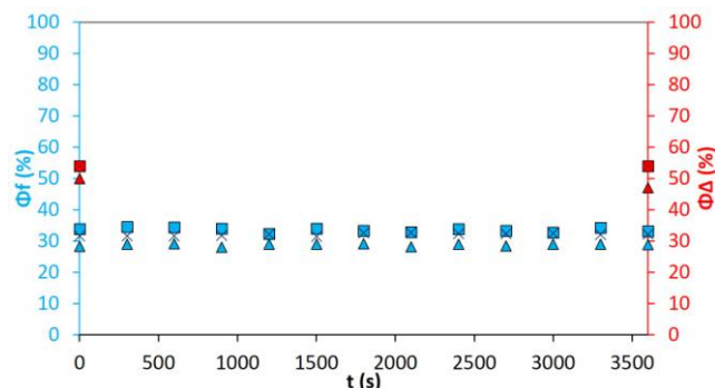
Figure 6. Evolution of \Phi_f and \Phi_\Delta quantum yields of compounds Pyro-a , 12 and 13 under light irradiation ( 668 nm, 10 mW \cdot cm^{-2} ) over time. Legend: ( \square ) Pyro-a , ( \Delta ) 12 , ( \times ) 13 .
