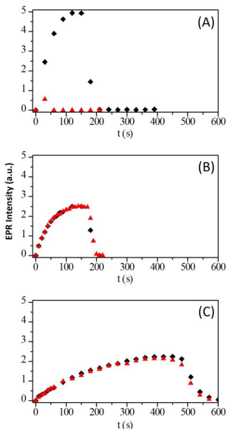
Figure 8. EPR intensity of radical generated after different irradiation time for Alk (A), 9 (B) and 13 (C) at 300 \mu\text{M} in methanol with ( \blacklozenge ) or without ( \blacktriangle ) oxygen.
