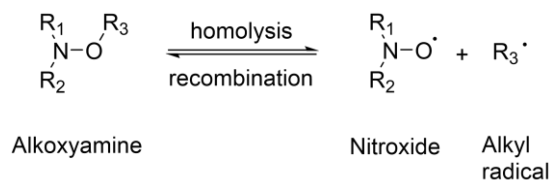
Scheme 1. Reversible \text{NO}-\text{R}_3 bond in alks.
