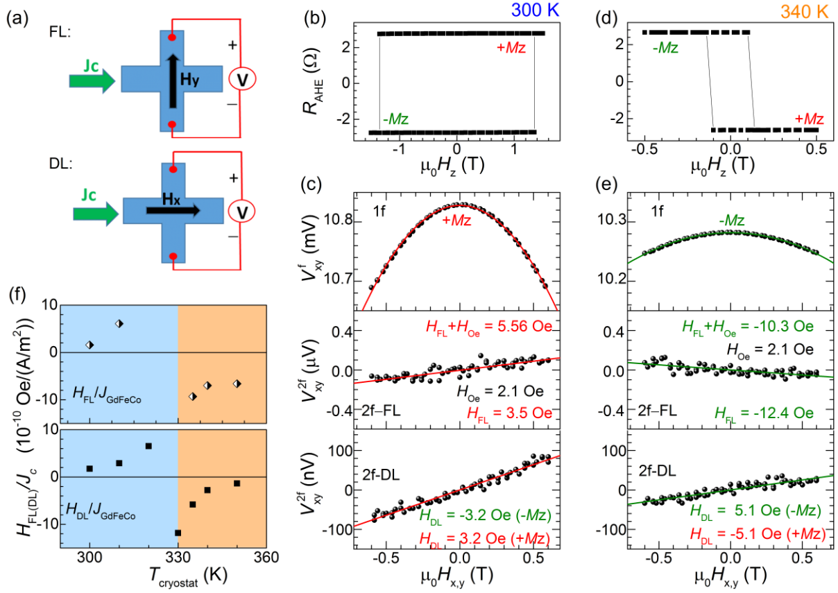
Figure 3. Self-torques in Gd 27 FeCo(10nm)/Cu(2nm). (a) Experimental configurations for second harmonic measurements. (b-f) AHE and second harmonic measurements for a GdFeCo(10 nm)/Cu(2 nm)/AlOx(2.5 nm) sample at 300 K (below T_M ) on left side (b-c) and 340 K (above T_M ) on right side (d-e). In (c) and (e) the symbols stand for experimental data while the red curves are the quadratic (linear) fits for the 1 st harmonic (2 nd harmonic). The results for the y (x) components H_{\text{FL}} ( H_{\text{DL}} ) of the FL (DL) fields for current along x are indicated in the Figures (for H_{\text{DL}} , different signs for M along + and - z). H_{\text{FL}} is given after correction for the current-induced Oersted field. (f) FL and DL efficiencies in the GdFeCo(10nm)/Cu(2nm)/AlOx(2.5nm) sample as a function of temperature (the magnetic compensation temperature T_M is indicated by color code). Both self-torques change sign across T_M (above T_M , H_{\text{DL}} is expected to go to zero at the angular momentum compensation temperature, see Supporting Information note S5 ).
