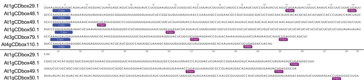
Figure 2. Characterization of FIB2-YFP snoRNP (A) Arabidopsis C/D-box protein orthologues (left) and C/D snoRNA (right) detected in the FIB2-YFP IP fractions using LC-MS/MS and RNA-seq approaches. The number of peptides and % of protein coverage for each protein is shown and the number of predicted 25S, 18S and 5.8S rRNA targets identified in the 5' and 3' antisense sequences of 141 C/D snoRNA. (B) Representation of 6 novel C/D snoRNA detected in the FIB2-IP fraction. C and D boxes are boxed. These C/D snoRNA do not contain a matching rRNA target sequence.
