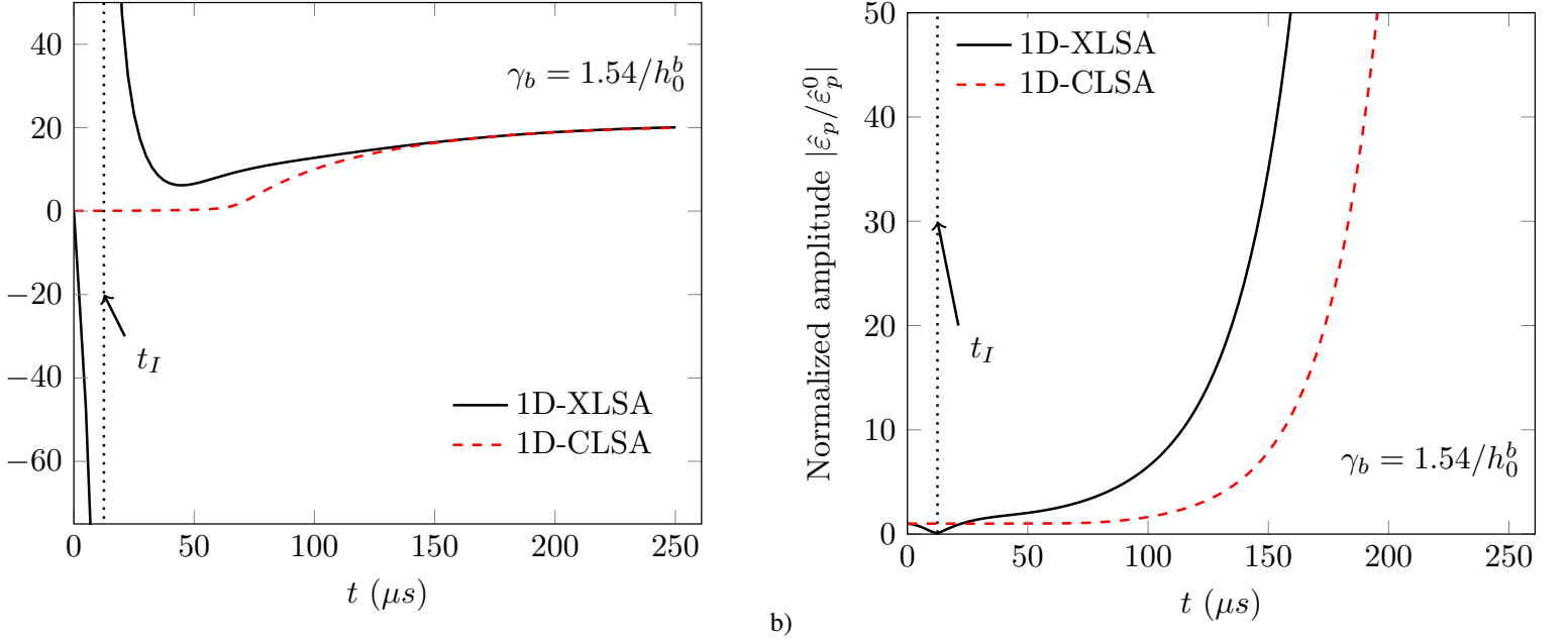
Figure 4: Time evolution of a) the normalized growth rate \eta_{\varepsilon_p}/\dot{\varepsilon}_0 and b) the normalized amplitude |\hat{\varepsilon}_p/\dot{\varepsilon}_0^p| for the 1D-XLSA model and for the 1D-CLSA model. Results are provided for the specific wavenumber \gamma_b . The vertical dashed line observed for time t_I is due to the observation that the predicted amplitude for the perturbation vanishes. The material is thermoviscoplastic, with a powerlaw flow stress, see Eq.(20). Material parameters are listed in Table 1. The nominal strain rate is 2300s^{-1} . Initial thickness is h_0^b = 2.4 mm . Initial amplitude of the thickness perturbation is \hat{h}_0 = 8 \mu m .
