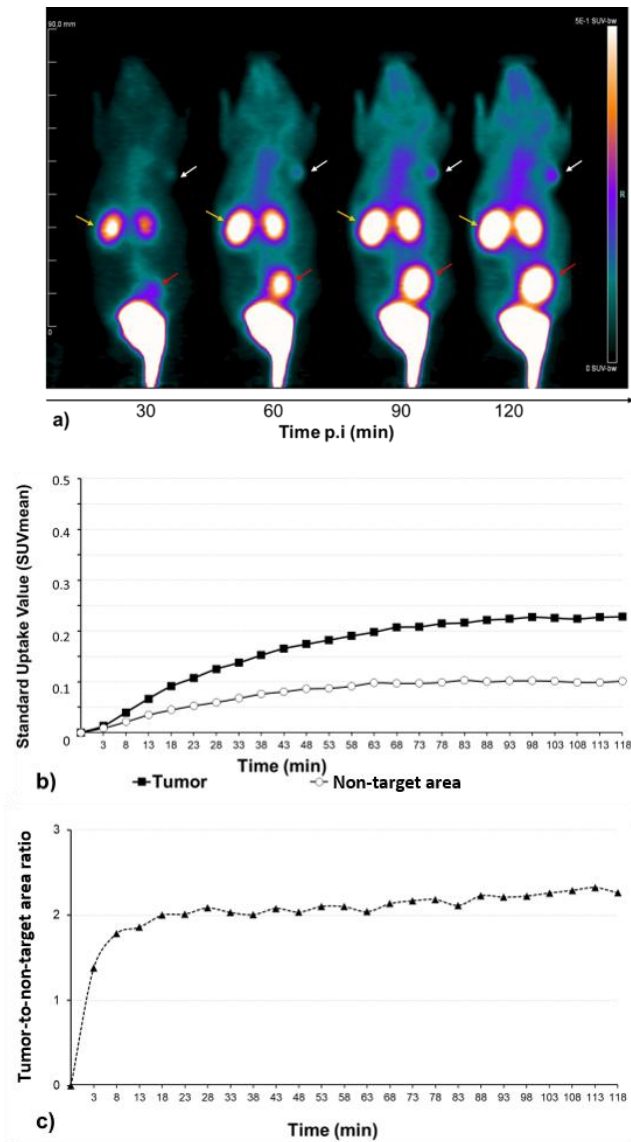
Fig. 2. (a) Dynamic PET images displayed through coronal sections and recorded during 120 min following [ ^{68}\text{Ga} ]13 injection in U87MG engrafted mice (n=3). Color scale is expressed in SUV values. The tumors are indicated with white arrows, the kidneys with yellow arrows and the bladder with red arrows. (b) Corresponding time-activity curves for mean SUV from tumor (black square) and from non-target area (white circle), as well as for tumor-to-non-target area ratio (black triangles) (c).
