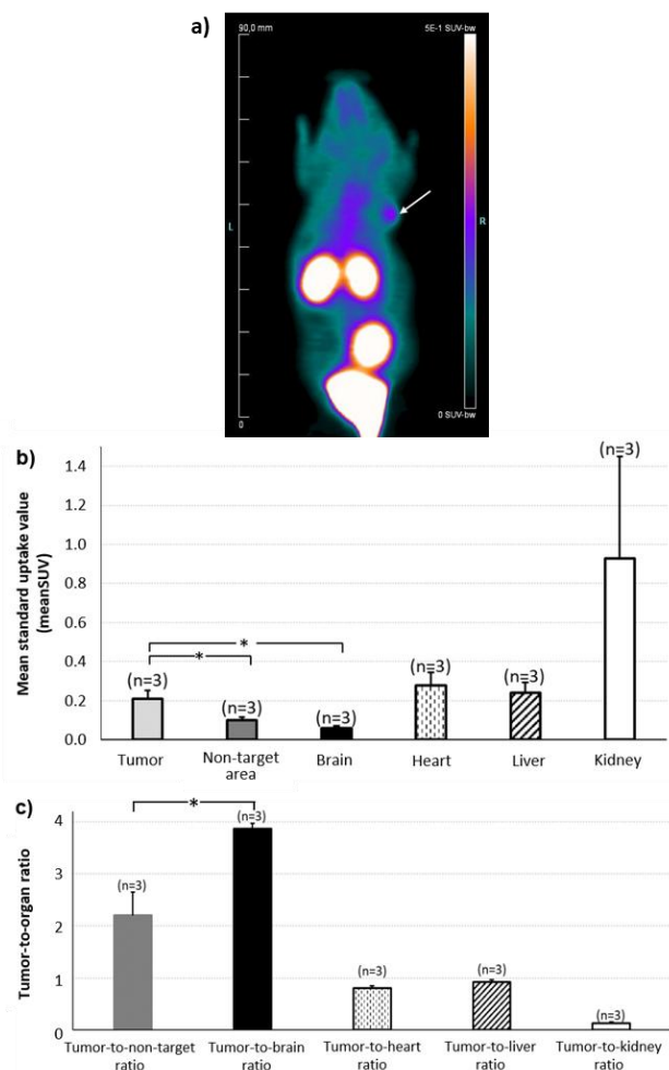
Fig 3. (a) Whole-body image of the 2 nd hour of PET recordings after [ 68 Ga]13 injection. (b) Results of SUVmean values obtained at the 2 nd hour of PET recording for tumors and various organs, after the injection of [ 68 Ga]13. (c) Comparison of tumor-to-organ ratio for activities measured during the 2 nd hour of PET recording. *: p < 0.05 . The tumor is indicated with white arrows and the color scale is expressed in SUV values ( n = 3 ).
