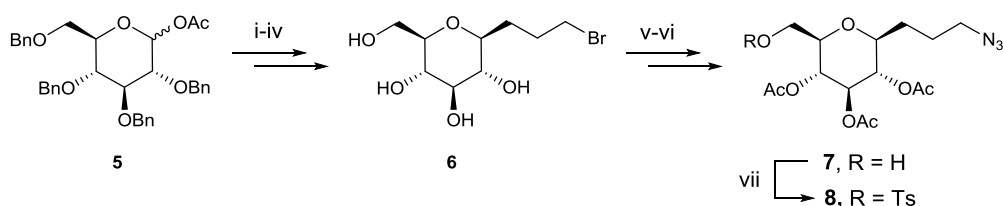
Scheme 2. C-glycoside derivative synthesis. Reagents and conditions: (i) TMSI, CH 2 Cl 2 , 0°C, 1h, then AllylMgBr, 0°C to rt, 3h, 90%; (ii) 1) 9-BBN, THF, Δ, 4h; 2) EtOH, NaOH, H 2 O 2 , 12h, 89%; (iii) PPh 3 , CBr 4 , CH 2 Cl 2 , 0°C, 1h, 90%; (iv) Pd(OH) 2 /C (20% w/w), THF/H 2 O (5/1 v/v), H 2 , 33 psi, 13h, 93%; (v) NaN 3 , acetone/water (5/1 v/v), reflux,
