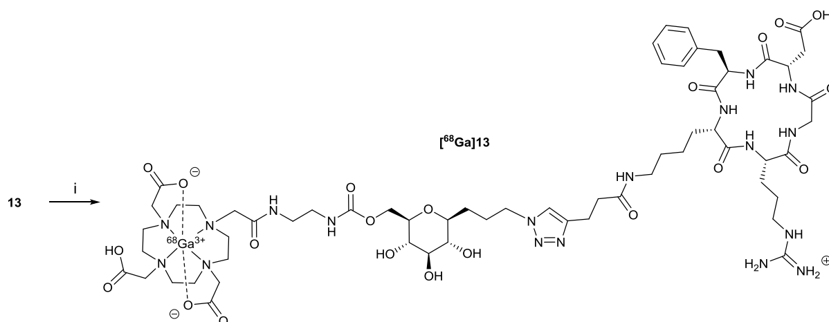
Scheme 4. Radiosynthesis of [ ^{68}\text{Ga} ]13. Reagents and conditions: (i) [ ^{68}\text{Ga} ]GaCl _3 , AcONa (0.7 M) 110°C, 10 min, 78 \pm 3% dc.
