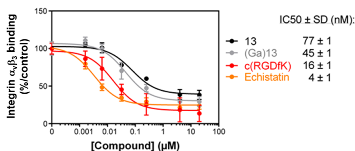
Fig. 1. Solid-phase binding assay. Effect of 13 (dark) and ( Ga13 ) (grey) on the binding of \alpha_v\beta_3 integrin onto vitronectin compared with two reference molecules: c(RGDfK) (red) and Echistatin (orange). IC_{50} values (nM) were calculated using one-site fit log- IC_{50} non-linear analysis regression (graphpad prism).
