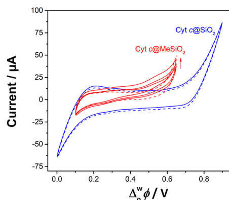
Figure 6. Cyclic voltammograms of Cyt c@SiO 2 (blue curve) and Cyt c@MeSiO 2 (red curves) modified ITIES in the absence (dashed curves) and in the presence (solid curves) of 100 \mu M DcMFC in the organic phase. They cyclic voltammetry was performed using electrochemical cell 4 (see Scheme 1) at a scan rate of 20 mV s -1 . The arrow represents the current evolution with the repetition of scans in the case of Cyt c@MeSiO 2 .
