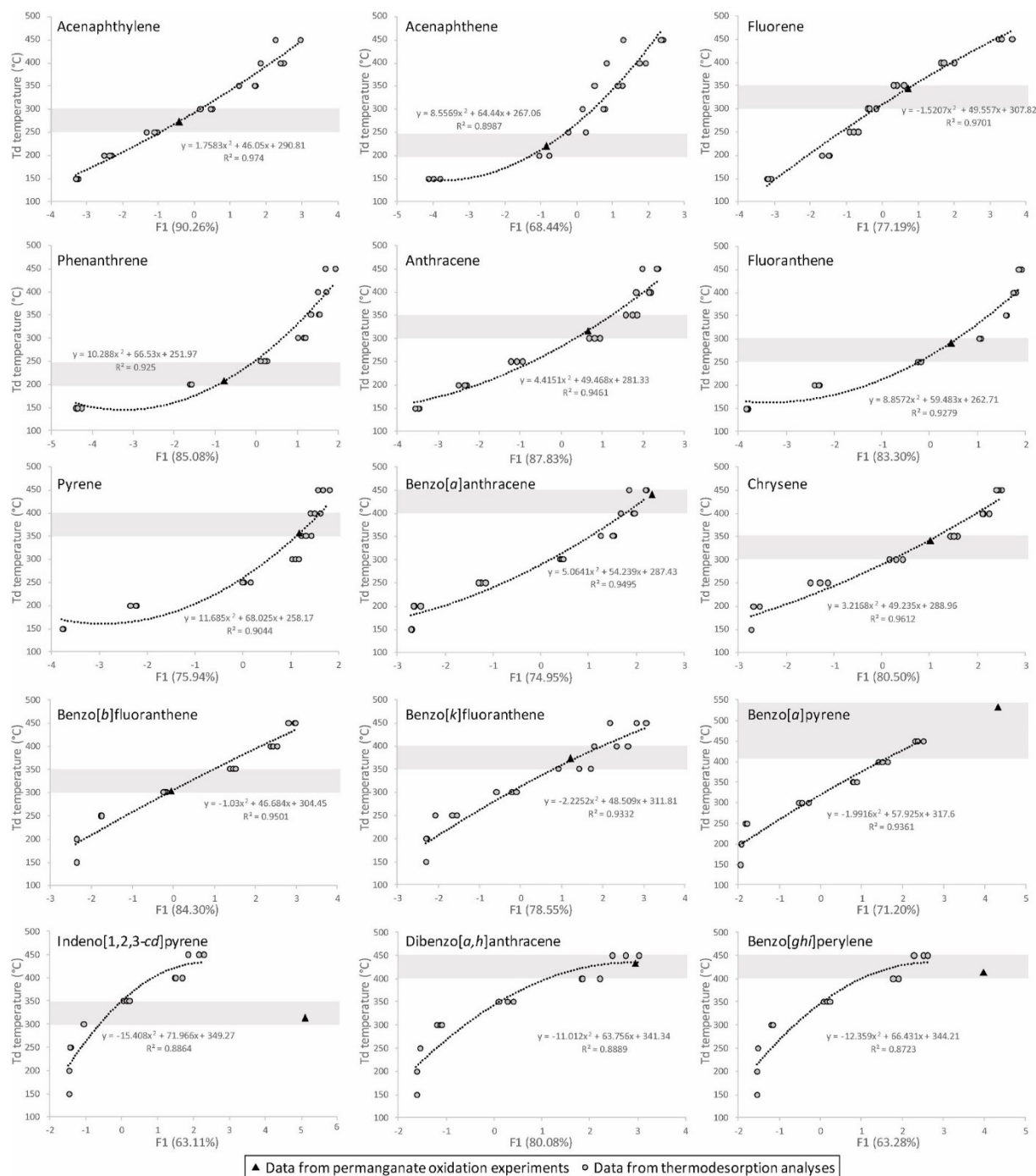
Fig. 3: Plot of the desorption temperature as a function of the F1 coordinate of the principal component analysis for the 15 PAHs degraded during KMnO_4 oxidation. The grey areas have been added to facilitate the reading of the desorption temperature of the oxidized samples.
