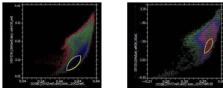
Figure 2: Scatter plots used to locate the disturbed pixels (example for year 2002 and 2007).
