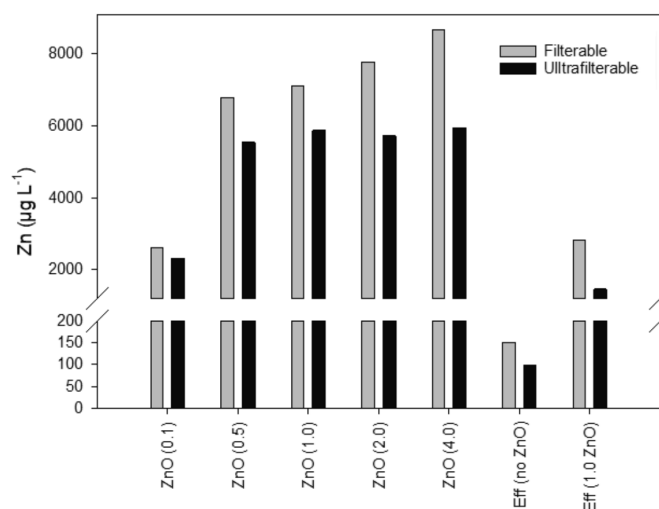
Figure 4. Total Zn recovery after filtration and ultrafiltration from distilled water spiked with 0.1 , 0.5 , 1 , 2 , and 4 \text{ g L}^{-1} ZnO and biologically treated wastewater (Eff) with ( 1.0 \text{ g L}^{-1} ZnO) and without Zn spiking.
