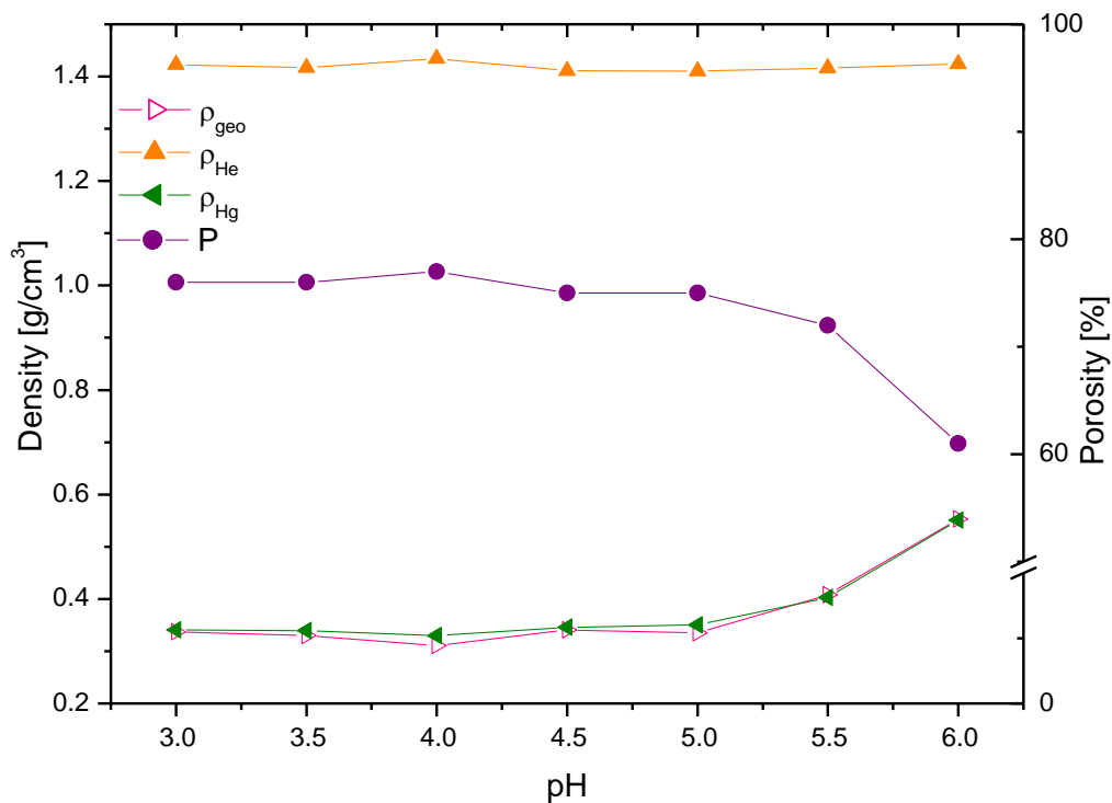
Figure 1. Relationship between different densities and porosities of the RF xerogels studied and the pH of their precursor solutions.
