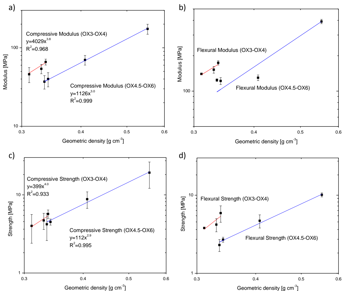
Figure 8. Mechanical properties of RF xerogels as a function of their geometric density, fitted by power laws.
