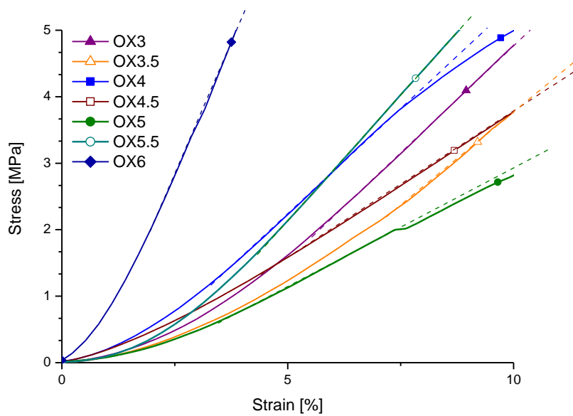
Figure S3. Linear elastic behaviour during the compressive tests of the OXs samples.
