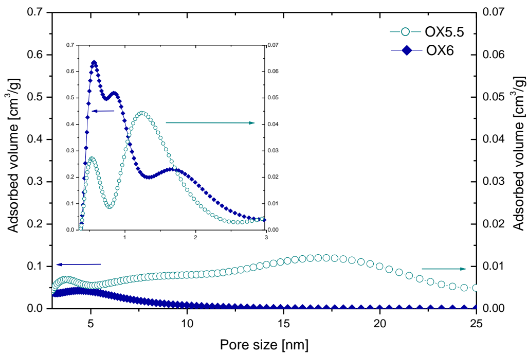
Figure S2. NLDFT pore size distributions calculated from \text{N}_2 adsorption isotherms.
