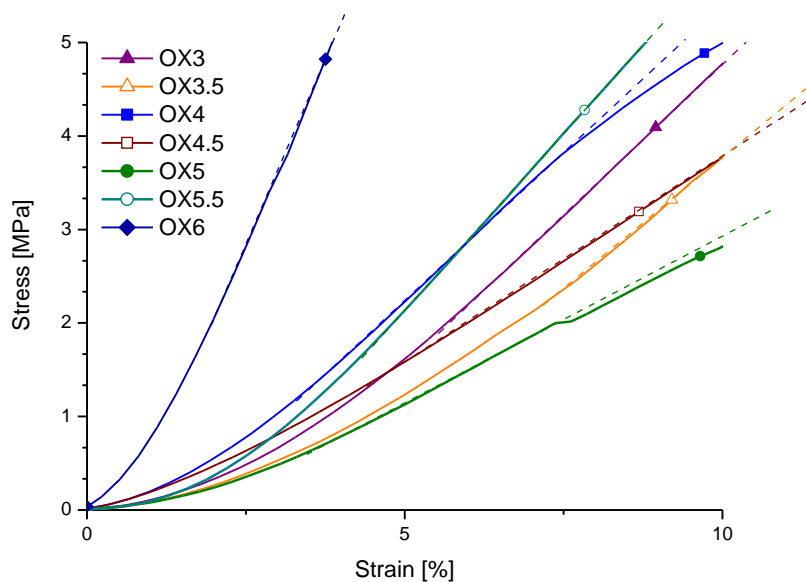
Figure S3. Linear elastic behaviour during the compressive tests of the OXs samples.
