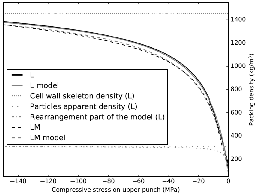
757 758 Figure 11. Compression model and experiments, considering that the cell wall density depends on 759 compressive stress ( K_s = 3.8 GPa).
