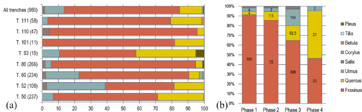
Figure 5. Charcoal assemblages (a) by trench, with the quantity of charcoal fragments used as base for the percentage values shown in parentheses, (b) and by chronological phase, with the average quantities of fragments per taxon per phase shown inside the bars.
