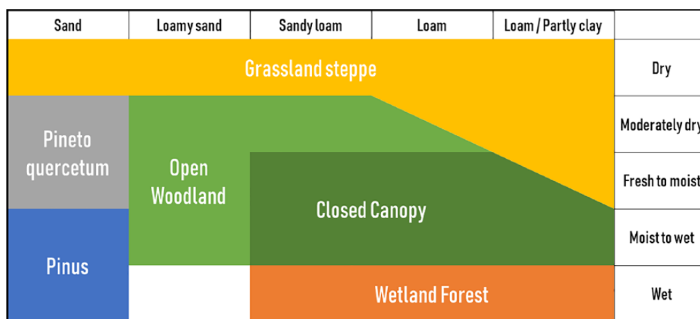
Figure 3. Ecogram of vegetation dependencies with respect to soil texture and moisture, based on information from Horvat et al. (1974) and Walter and Breckle (1997).
