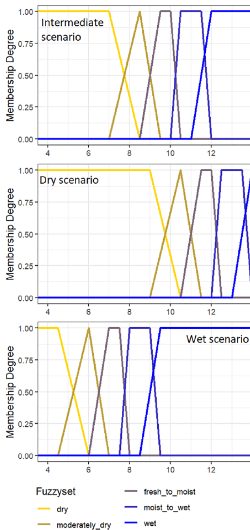
Figure 4. Membership of the fuzzy sets defining the wetness of the soil based on the terrain wetness index for intermediate, dry, and wet scenarios.
