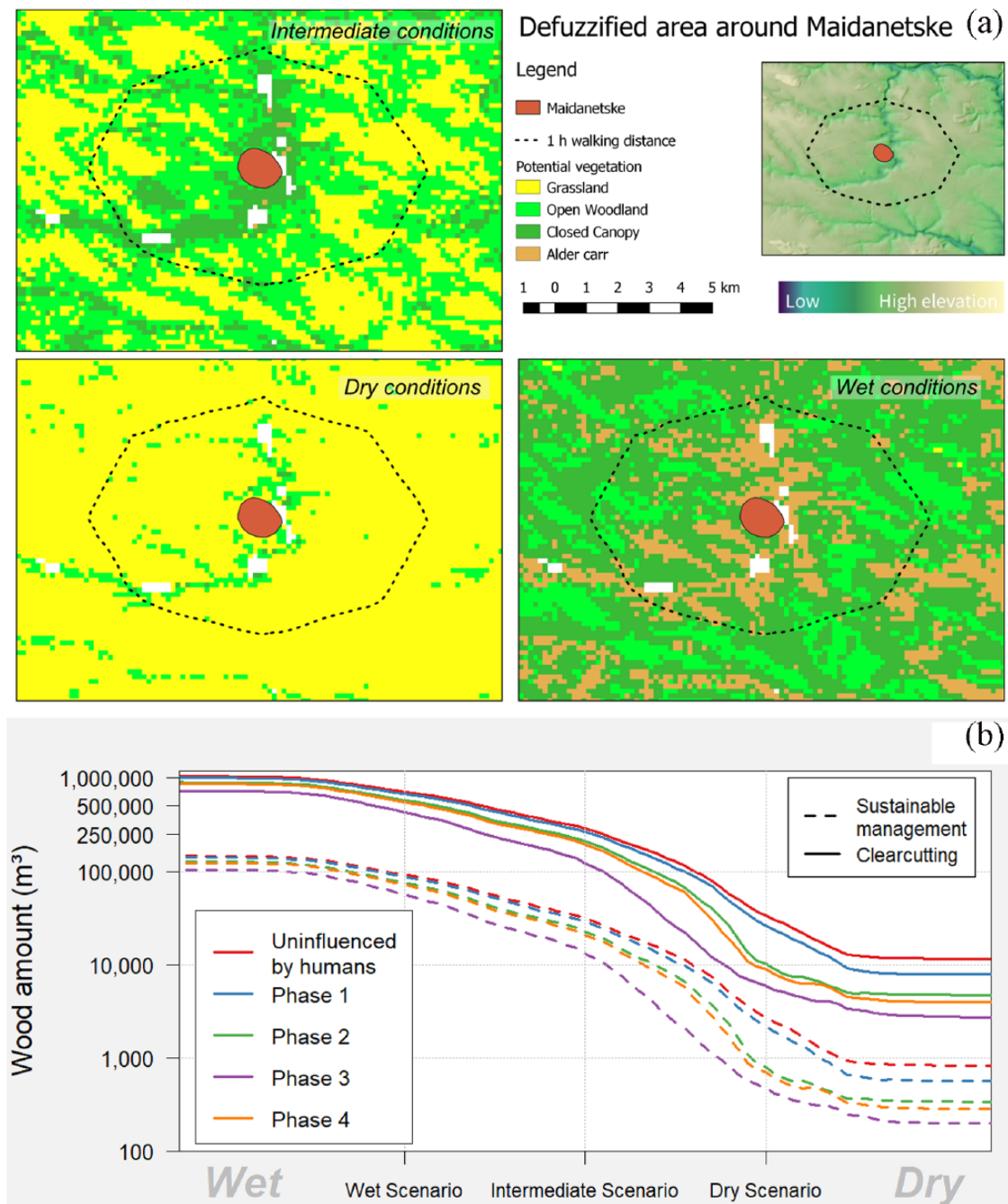
Figure 7. (a) Defuzzified simulation of the vegetation close to Maidanetske and (b) fuzzified simulation of amount of wood available close to Maidanetske.
