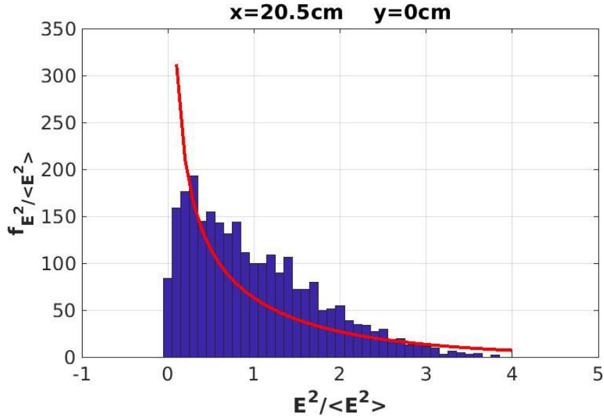
Рис. 13: The intensity distributions, blue histogram is the numerical distribution, red curve is the analytical distribution normalized to the number of realizations. Turbulence level \frac{\delta \tilde{n}_{max}}{n_{max}} = 5.0\% , radial position x = 20.5 cm at axis of the average beam
