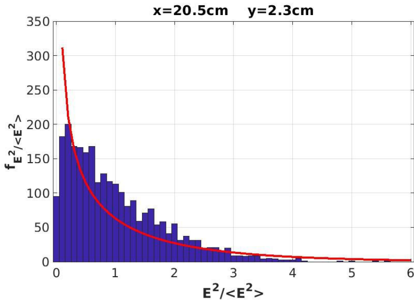
Рис. 14: Intensity distributions, blue histogram is the numerical distribution, red curve is the analytical distribution normalized to the number of realizations. Turbulence level \frac{\delta \tilde{n}_{max}}{n_{max}} = 5.0\% , radial position x = 20.5 cm at width of the average beam y = 2.3 cm
