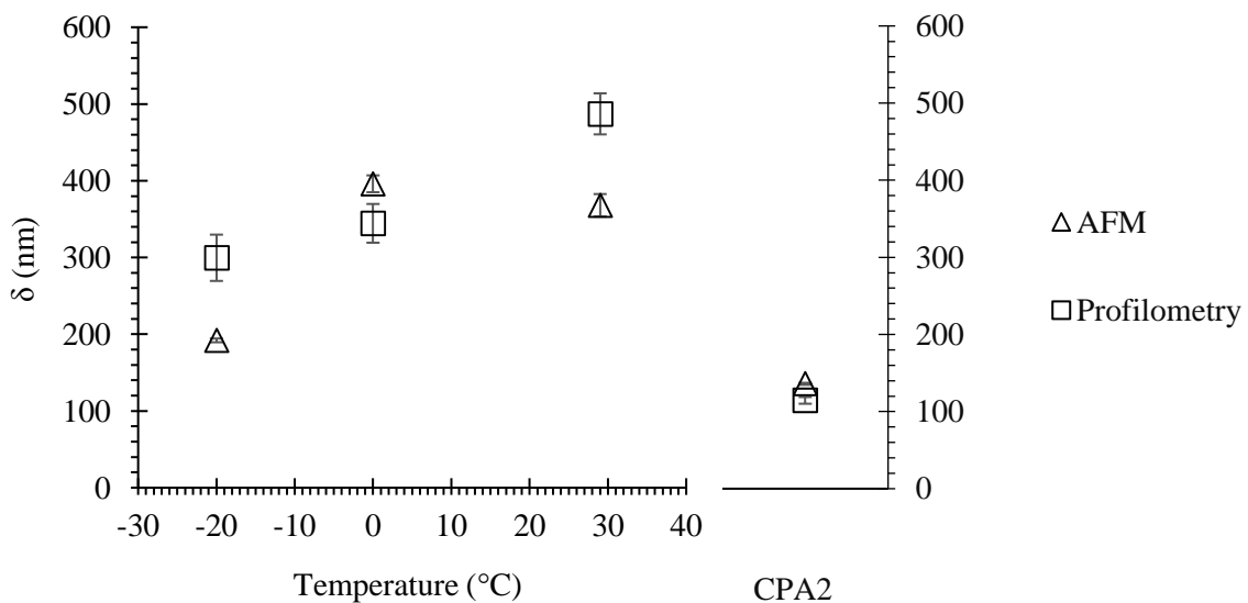
Figure 7. Top-surface thickness analysis via profilometry and AFM for Syn -20 °C, Syn 0 °C, Syn 29 °C and CPA2 samples.
