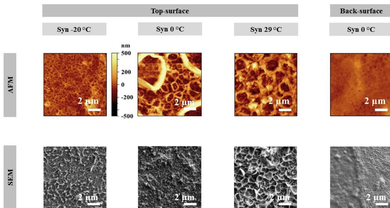
Figure 3. AFM and SEM images of synthesized APA films' top-surface and back surface
