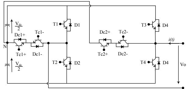
Fig. 2 HB-T-type five level topology.
