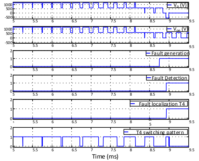
Fig. 9 Simulation results when T4 is faulty (OCF).
