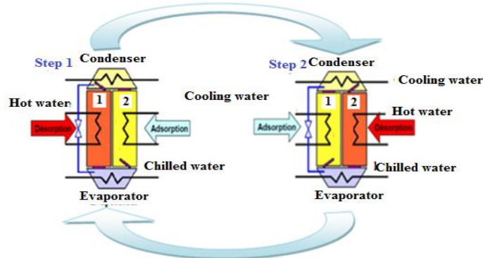
Figure 2: Schematic diagram of two bed solar-powered adsorption chiller.
