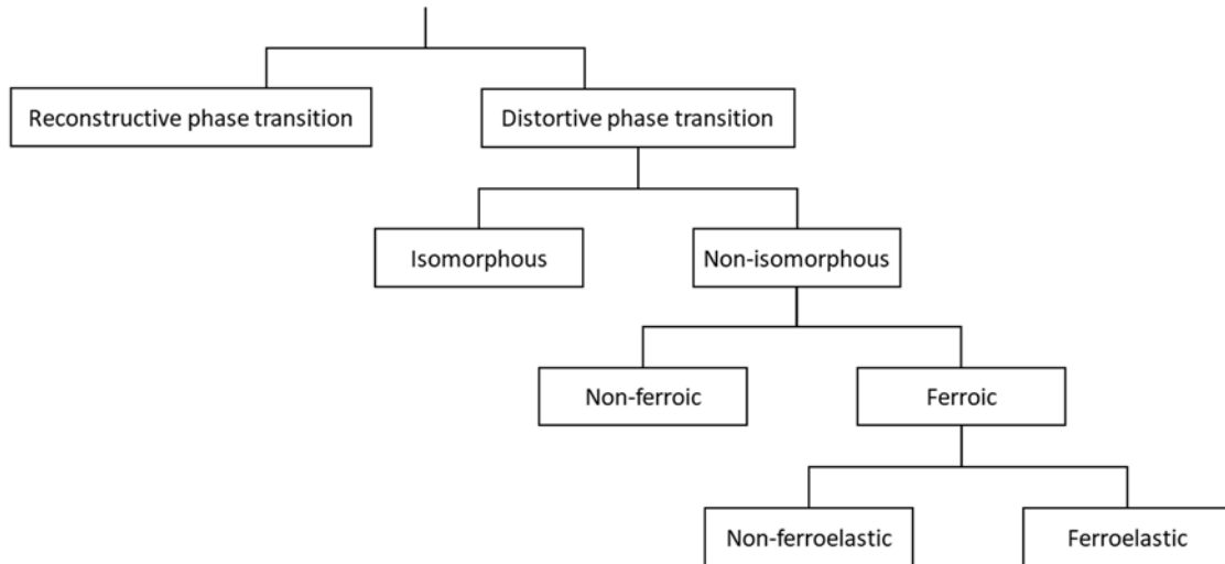
FIG. 10. Classification of structural phase transitions in SCO materials based on the symmetry reduction from the prototype phase to the daughter phase.
