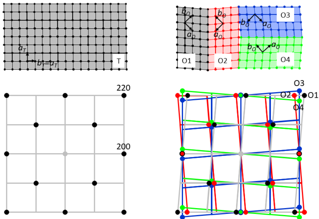
FIG. 12. (top) Schematic of the crystal lattices in the parent tetragonal phase (space group I4/mmm ) and in the orthorhombic daughter phase (space group Fmmm ) associated to the formation of four domain states (labelled O1, O2, O3, O4). Domain walls are identified between the different domains. (bottom) Schematic of the transformation of the single-crystal X-ray diffraction pattern during orthorhombic distortion and domain formation. Notice the diffraction peak splitting in the symmetry
