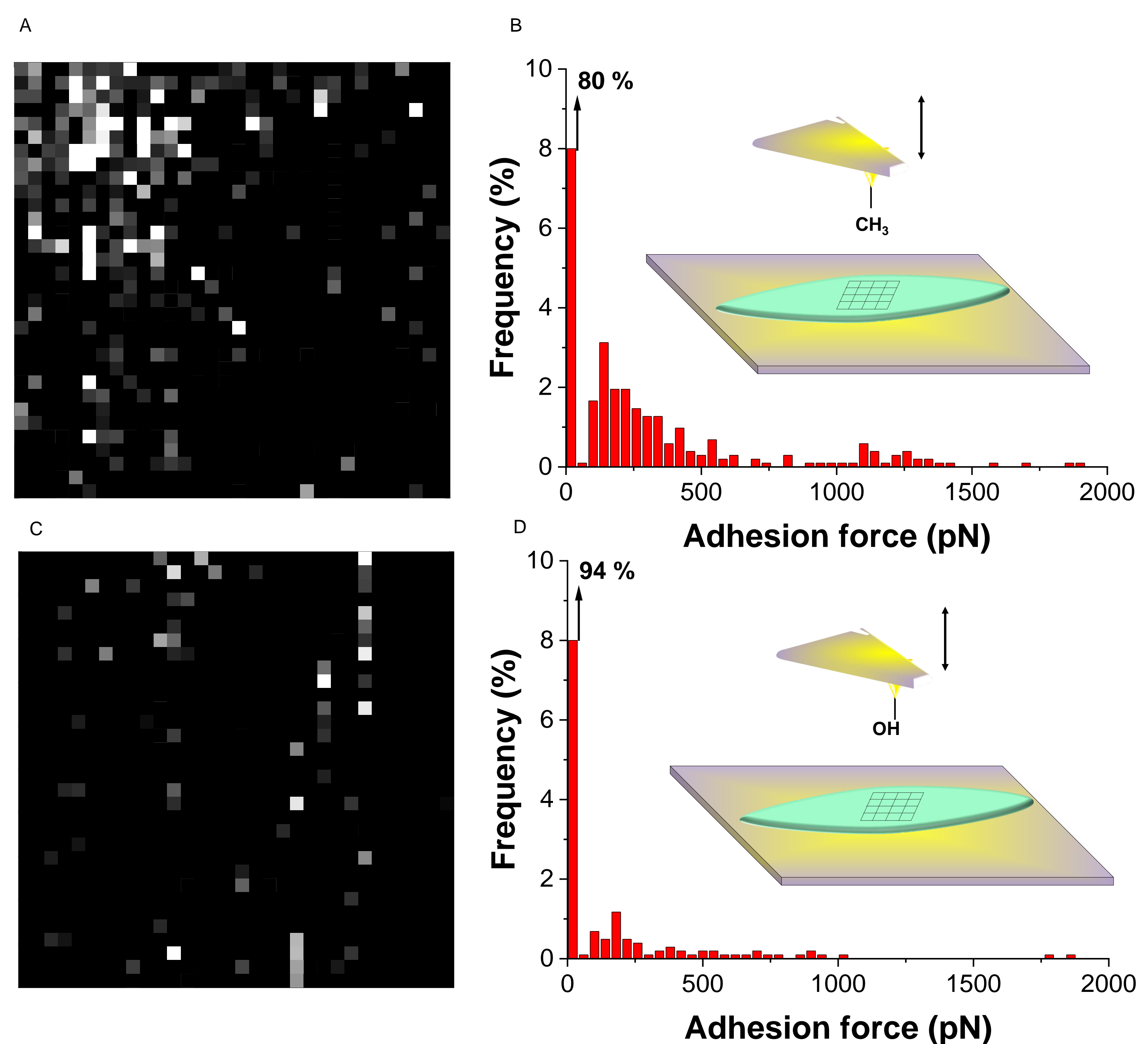
Figure 4 (single-molecule analysis): Adhesion force maps (2 x 2 \mu\text{m} ; z range = 1 nN) recorded with hydrophobic (A) or hydrophilic tips (C) at the surface of N. palea cells maintained in liquid medium and corresponding last rupture peak histograms (B, D)
