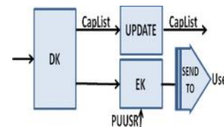
Figure 7.b: Sending the decryption parameters to the User
