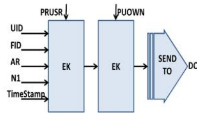
Figure 6: Sending a registration request to DO
