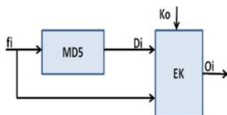
Figure 2: The ith file and its message digest (generated with MD5) are encrypted with DO symmetric key.
