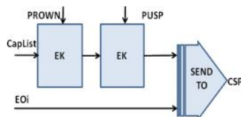
Figure 5: Securing and sending the CapList to CSP.
