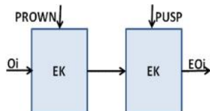
Figure 3: Successive encryption with DO key and CSP public key to establish authentication and confidentiality.
