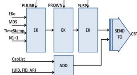
Figure 7.a: Updating and sending the CapList to CSP.
