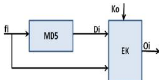
Figure 2: The ith file and its message digest (generated with MD5) are encrypted with DO symmetric key.
