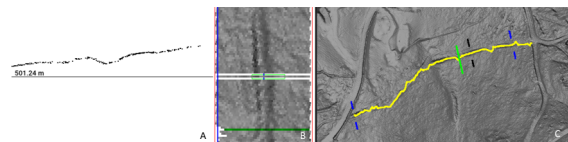
A: example of ground point profile used to detect a linear structure, here a holloway. B: processed adjacent profile aligned on the tracked structure center line. C: detected structure superimposed to the digital terrain model (in green, the manual initial scan; in black, the currently analysed profile; in blue, selected bound profiles for volume estimation)
