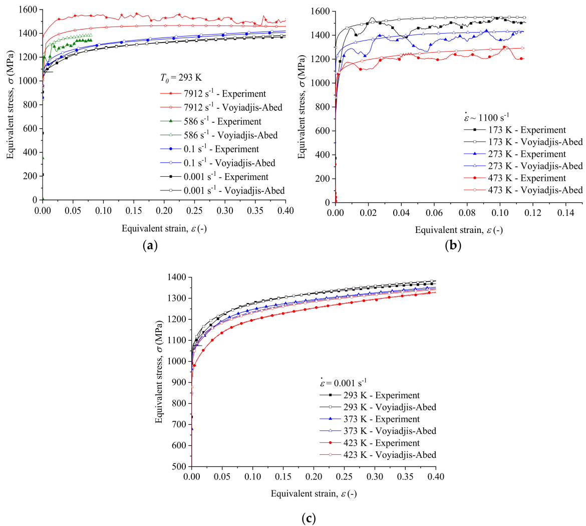
Figure 13. Comparison of the original Voyiadjis–Abed model and the experimental data: (a) for different strain rates, at T_0 = 293 K; (b) for different temperatures, at \dot{\varepsilon} \sim 1100 s^{-1} ; and (c) for different temperatures, at \dot{\varepsilon} = 0.001 s^{-1} .
