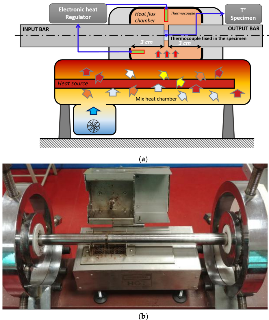
Figure 2. Description (adapted from [21]) (a) and picture (b) of the furnace used for high temperature dynamic compression tests.
