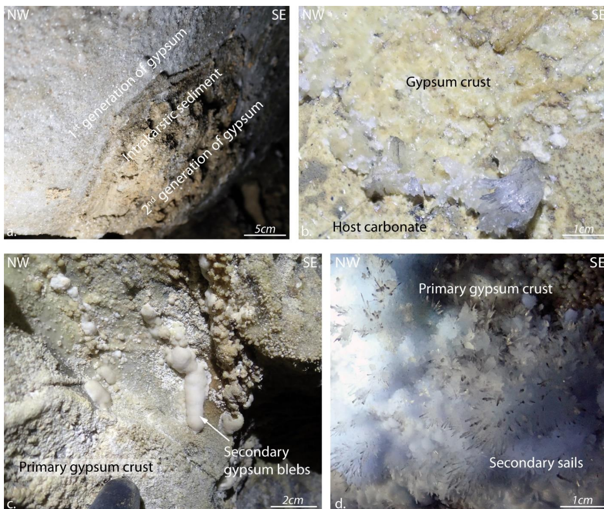
Figure 8: Photos of gypsum precipitates in the Ermite Cave. a. Two generations of gypsum crusts separated by a layer of clay-rich karstic sediments. b. Detailed view of the gypsum crust resting directly on the host limestone. c. Secondary gypsum blisters resting on the primary massive gypsum crust. d. Secondary fine gypsum needles on primary gypsum crust.
