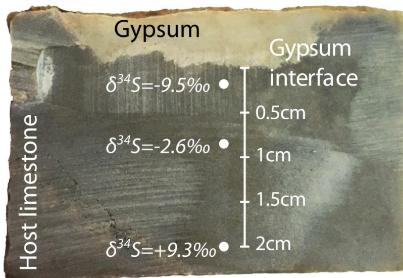
Figure 11: Photo of the interface between cave gypsum and host limestone in the Ermite Cave, indicating the position of samples and \delta^{34}\text{S} values (in ‰ V-CDT) of trace sulfate minerals used to identify the carbonate-gypsum substitution front.
