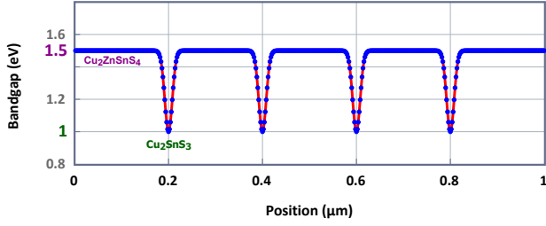
FIG. 5: The periodic inverted Gaussian profile used to model the variation of the bandgap with position in the CZTS alloy based on the \text{Cu}_2\text{ZnSnS}_4 / \text{Cu}_2\text{SnS}_3 phase separation fraction. The bandgap of \text{Cu}_2\text{ZnSnS}_4 is \approx 1.5 eV, while the bandgap of \text{Cu}_2\text{SnS}_3 is \approx 1 eV. The fraction between the secondary \text{Cu}_2\text{SnS}_3 phase and the main \text{Cu}_2\text{ZnSnS}_4 phase is \zeta = 0.16 . The same type of function is used for the other parameters, viz. the affinity, permittivity, and density of states.
