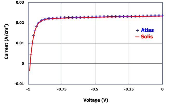
FIG. 4: The current-voltage characteristic of the single phase CZTS solar cell under the illumination by the AM1.5 spectrum. The voltage is applied to the top contact of the n-p structure. The symbols indicates the characteristic simulated using Atlas ® from Silvaco ® , while the straight line shows that simulated by Solis. The photovoltaic performance obtained by Solis and Atlas ® is presented in Table III.
