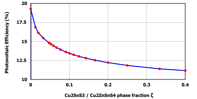
FIG. 7: The variation of efficiency of the multiple-phase CZTS solar cell with \zeta , the fraction between the secondary \text{Cu}_2\text{SnS}_3 phase and the main \text{Cu}_2\text{ZnSnS}_4 phase in the absorber.
