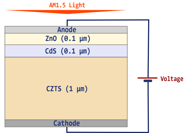
FIG. 2: The ZnO/CdS/CZTS solar cell structure. The ZnO and CdS layers are n-doped with a donor concentration of 10^{18} \text{ cm}^{-3} . The CZTS p-doping concentration is equal to 10^{16} \text{ cm}^{-3} .
