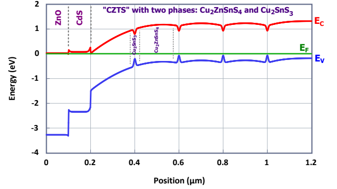
FIG. 6: The ZnO/CdS/CZTS band diagram at thermodynamic equilibrium for the multiple-phase CZTS absorber.
