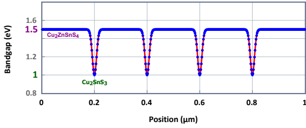
FIG. 5: The periodic inverted Gaussian profile used to model the variation of the bandgap with position in the CZTS alloy based on the \text{Cu}_2\text{ZnSnS}_4 / \text{Cu}_2\text{SnS}_3 phase separation fraction. The bandgap of \text{Cu}_2\text{ZnSnS}_4 is \approx 1.5 eV, while the bandgap of \text{Cu}_2\text{SnS}_3 is \approx 1 eV. The fraction between the secondary \text{Cu}_2\text{SnS}_3 phase and the main \text{Cu}_2\text{ZnSnS}_4 phase is \zeta = 0.16 . The same type of function is used for the other parameters, viz. the affinity, permittivity, and density of states.
