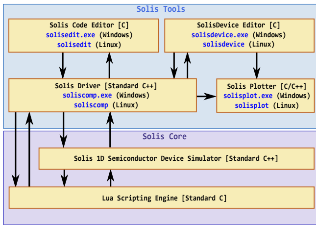
FIG. 1: The Schematic Solis architecture. The core part of Solis is entirely coded in standard C++ (the Lua engine being coded in standard C) and is easily portable to almost all operating systems, in addition to the natively supported Windows and Linux systems. The Solis code editor, device editor, and data plotter are developed in C and use the IUP GUI toolkit coded in C [9] and the Scintilla component coded in C++ [10].
