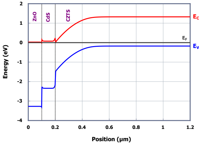
FIG. 3: The ZnO/CdS/CZTS band diagram at thermodynamic equilibrium.
