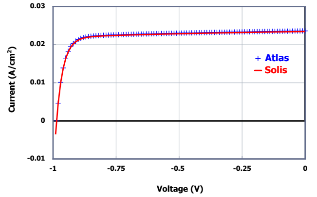
FIG. 4: The current-voltage characteristic of the single phase CZTS solar cell under the illumination by the AM1.5 spectrum. The voltage is applied to the top contact of the n-p structure. The symbols indicates the characteristic simulated using Atlas ® from Silvaco ® , while the straight line shows that simulated by Solis. The photovoltaic performance obtained by Solis and Atlas ® is presented in Table III.
