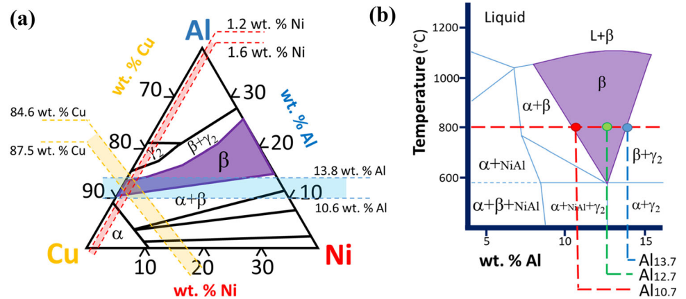
Fig. 1 CuAlNi ternary phase diagrams; a isothermal section at 800 °C, b pseudo-binary phase diagram at 2 wt.% Ni
