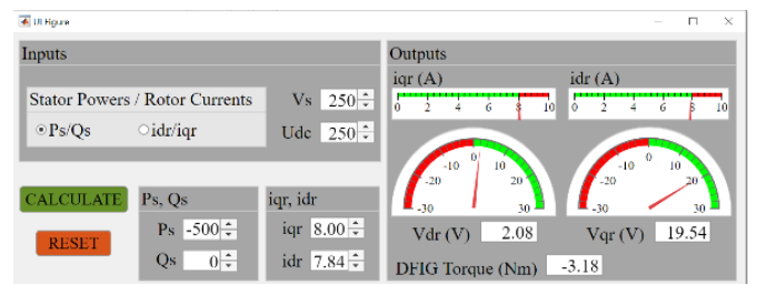
Figure 7. DFIG steady-state App interface for Q_s^* = 0 VAR
