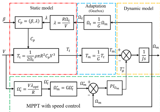
Figure 12. TSR based MPPT algorithm block diagram
