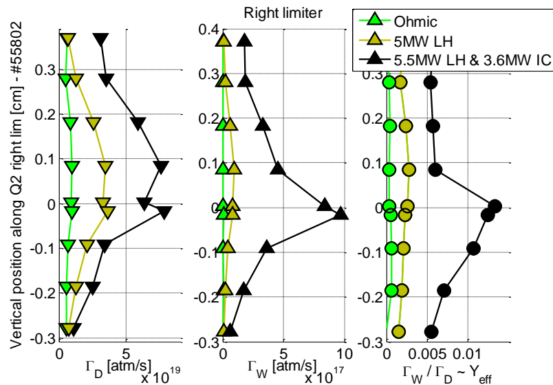
FIG 14: Deuterium and tungsten fluxes estimated from \text{DI}_\delta and \text{WI} calibrated data ( \text{Ph/m}^2/\text{s}/\text{sr} ) poloidal profiles along Q2 antenna right limiter with S/XB coefficients determined in section 1.2. Green and yellow profiles are the same as in Fig.12, and black profiles correspond to the last part of the same discharge with 5.5MW LH and 3.6MW ICRF power, characteristic of WEST high-power L-mode discharges.
