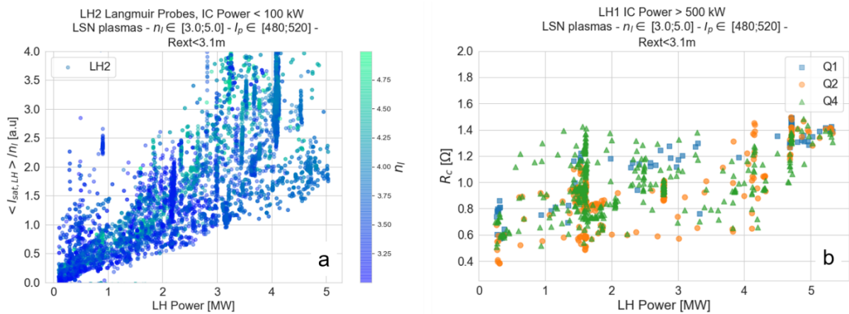
FIG. 7. (a) Ratio of ion saturation current measured by Langmuir probes fixed on LH2 launchers corners (a proxy for SOL density) over the line integrated density ( n_i ) from interferometry (proportional to core density) as a function of LH power. Only discharges from 2018 and 2019 with low ICRF power P_{\text{ICRF}} < 100 \text{ kW} , 3 < n_i < 5 \cdot 10^{19} \text{ m}^{-2} , 480 < I_p < 520 \text{ kA} and R_{\text{ext}} < 3.1 \text{ m} were selected and (b) ICRF antennas average coupling resistances as a function of the LH power.
