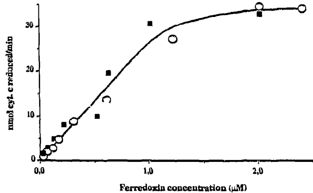
Fig. 4. Ferredoxin-dependent reduction of cytochrome c by ferredoxin-NADP reductase. Ferredoxin-NADP reductase concentration in the cuvettes was 40 nM. Cytochrome c reduction was followed at 550 nm at 30°C (■, native ferredoxin protein; ○, recombinant protein).
